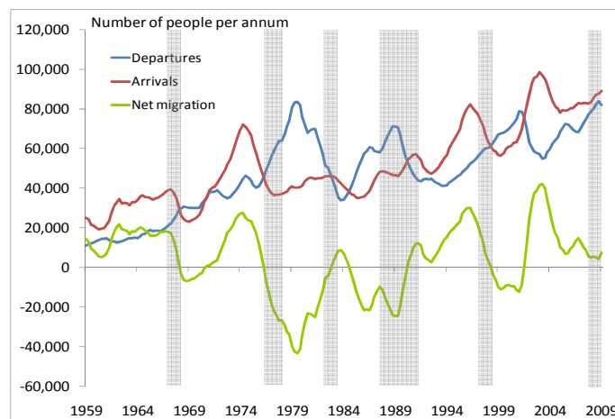
Fig 3: Annual PLT net migration, arrivals and departures
